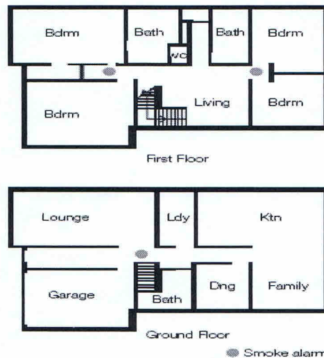
Diagram 3: Two storey dwelling showing smoke alarms in the storey containing bedrooms (first floor) and the storey not containing bedrooms (ground floor)
