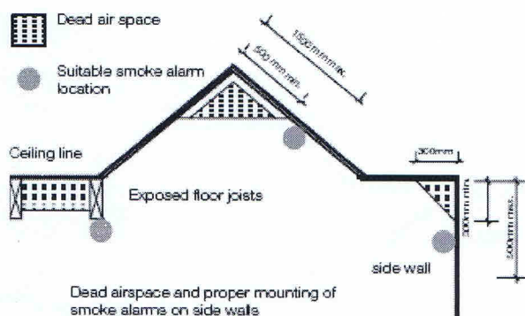
Diagram 7: Proper mounting of smoke alarms
